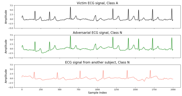
Figure 2: Adversarial Attack v.s. Substitution attack
