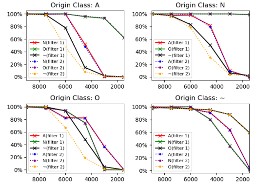
Figure 4: Success attack rates with different sized windows.
